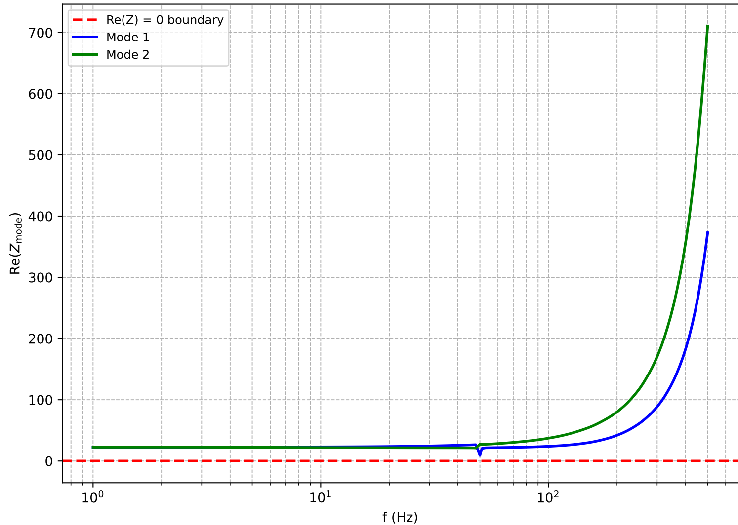
Real part of modal impedances vs frequency
